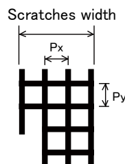
Clearance of each grid mm tangential direction : P_x=0.4 radial direction : P_y=0.4 Details of Scratches
