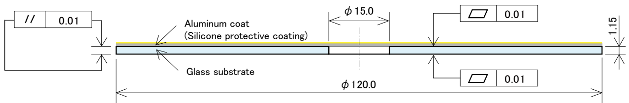
Dimensional drawing of SCD-4143
