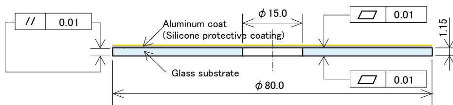
Dimensional drawing of SCD-4142
