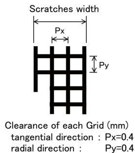
Details of Scratches
